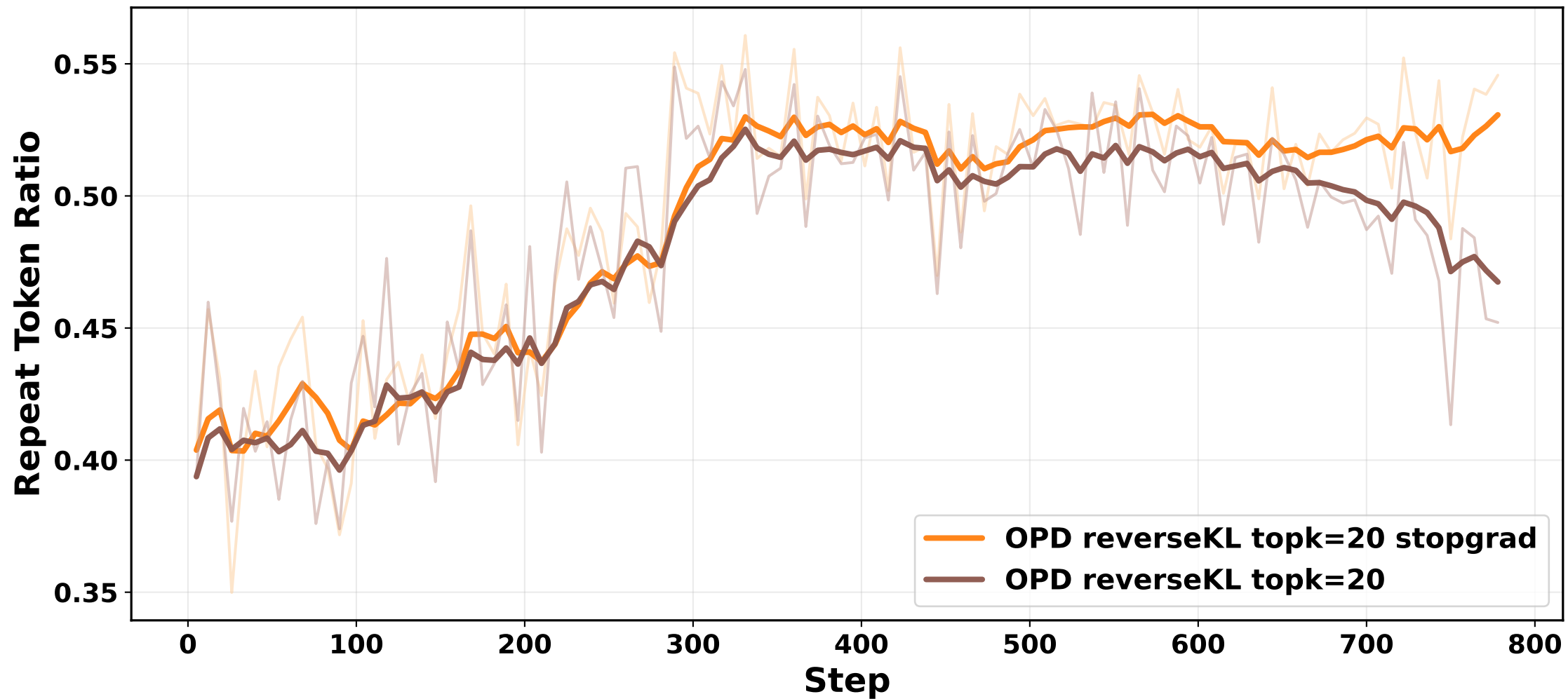
train/repeat_ratio
